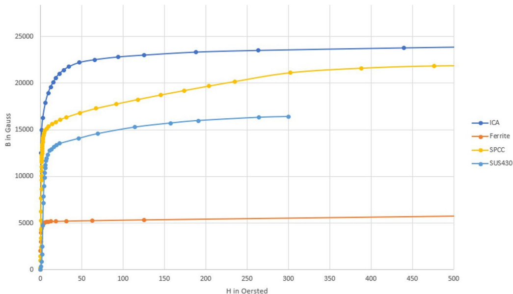
Figure 6-1: Material BH Curves
