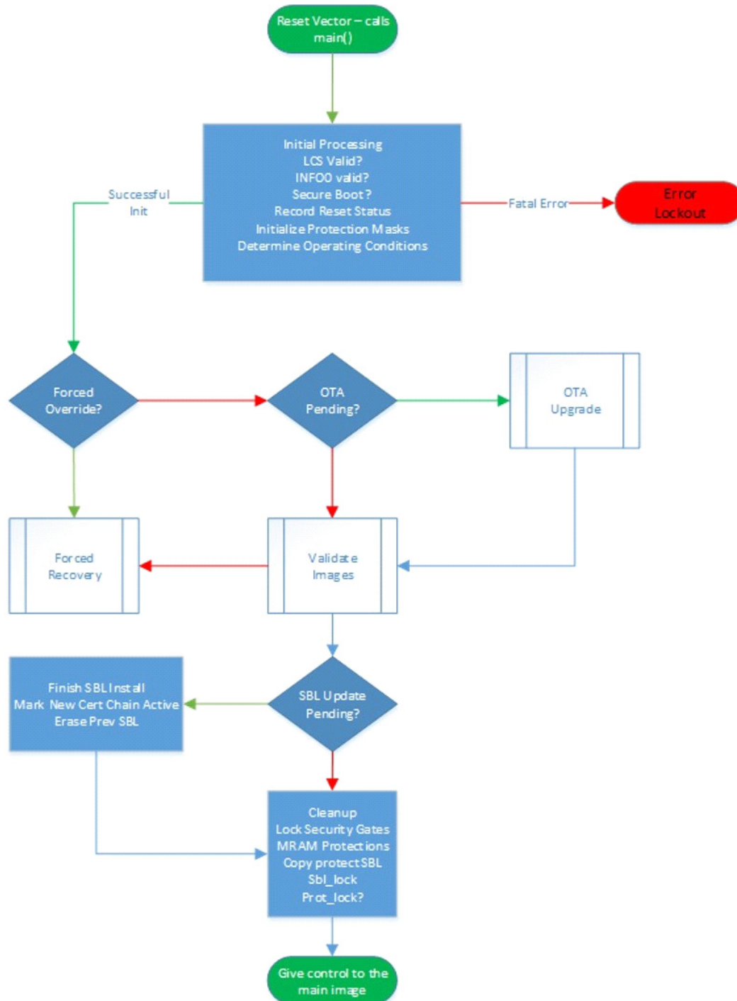
Figure 2. Secure Boot Loader (SBL) Flow
