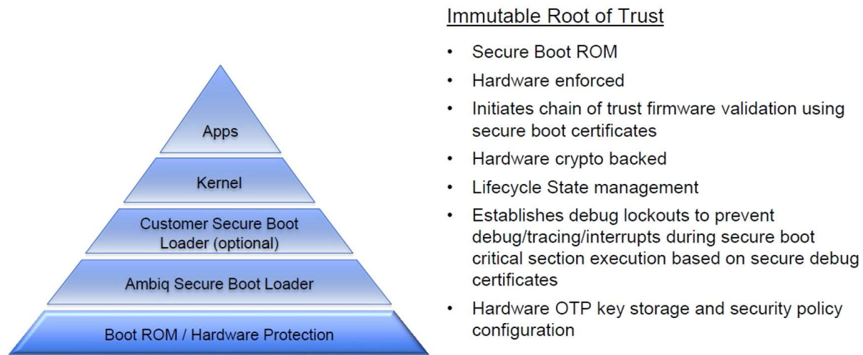
Figure 1. Apollo5 Secure Boot Architecture
