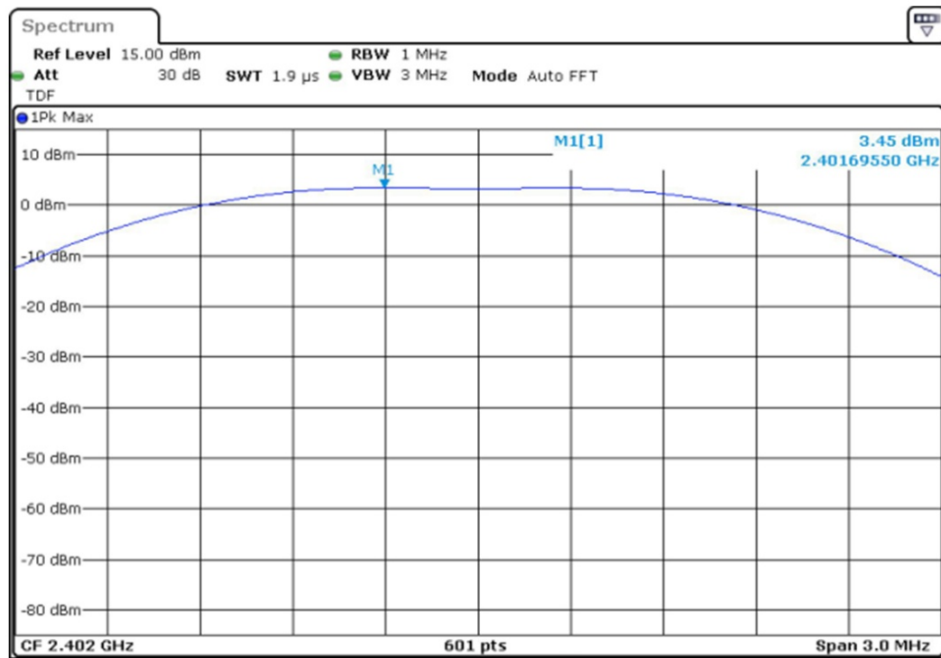
Figure 7-1: Example Test Plot of Maximum Conducted Output Power
