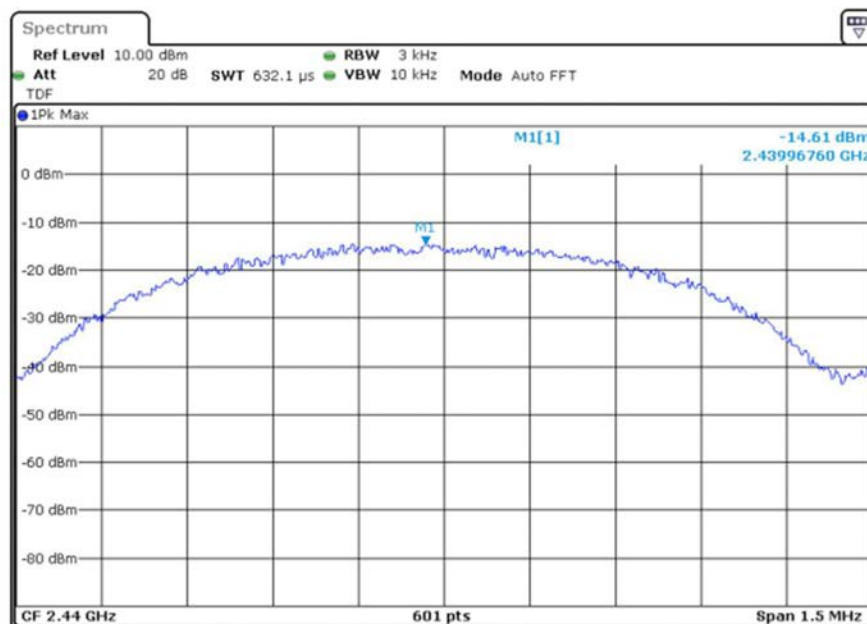
Figure 7-12: Example Test Plot of Power Spectral Density in Mid Channel
