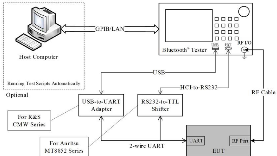
Figure 5-1: The Test Setup for Bluetooth Low Energy Signaling Test Method
