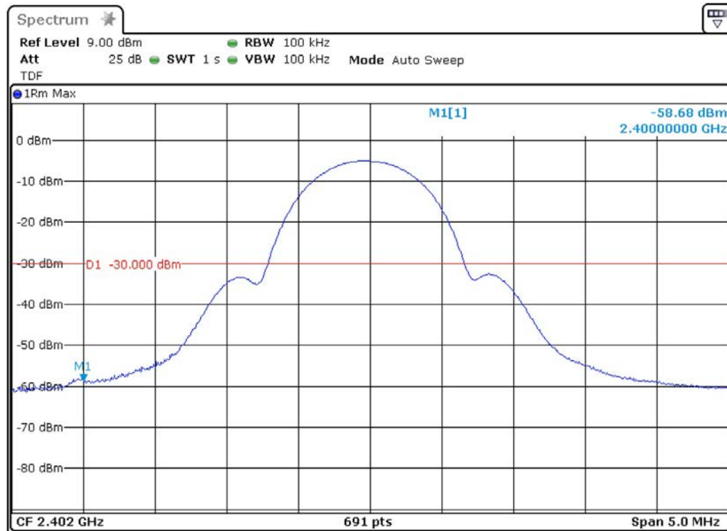
Figure 6-3: Example Test Plot of Frequency Range Testing
