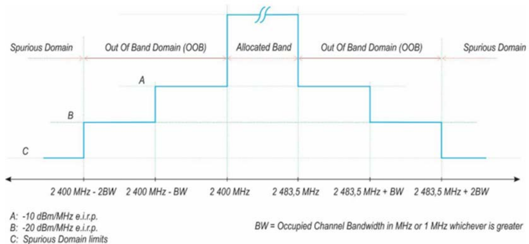
Figure 8-4: Transmit Mask
