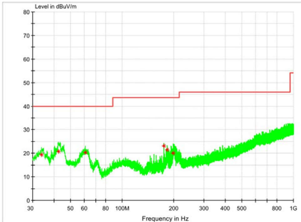
Figure 7-8: Radiated Emission Test Plot for 30 MHz to 1 GHz
