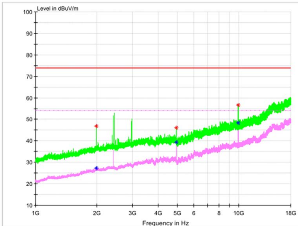
Figure 7-9: Radiated Emission Test Plot for Above 1 GHz
