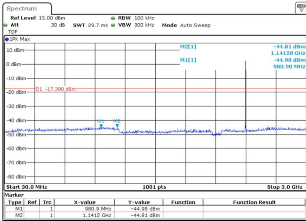
Figure 7-4: Example of Conducted Spurious Emission Test for 30 MHz to 3 GHz
