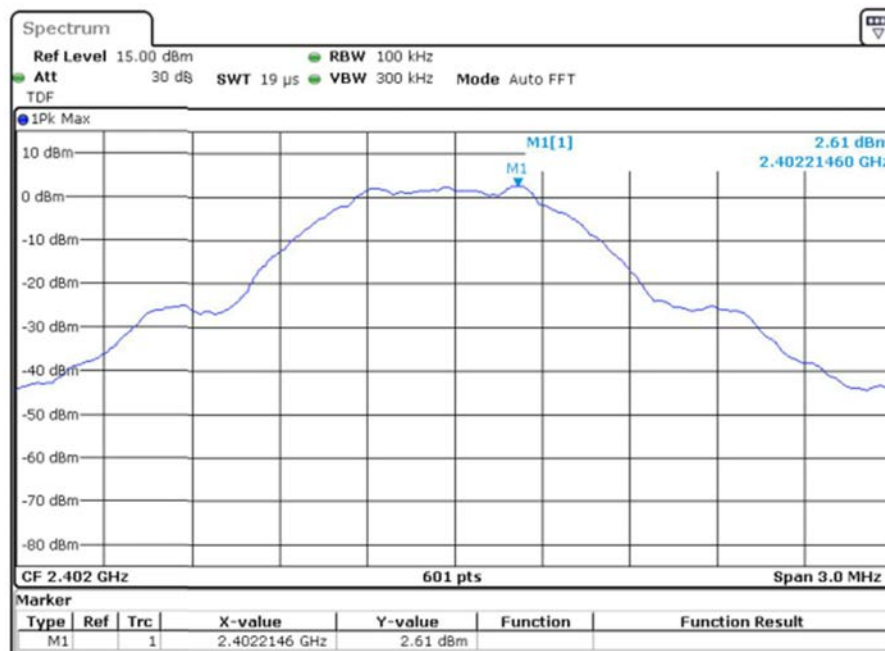
Figure 7-10: Reference Level of Fundamental Emission Testing in Low Channel
