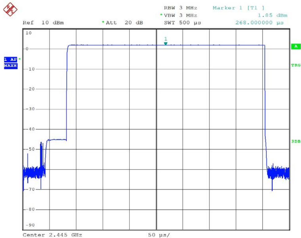
Figure 8-2: Example Test Plot of RF Output Power at Middle Channel
