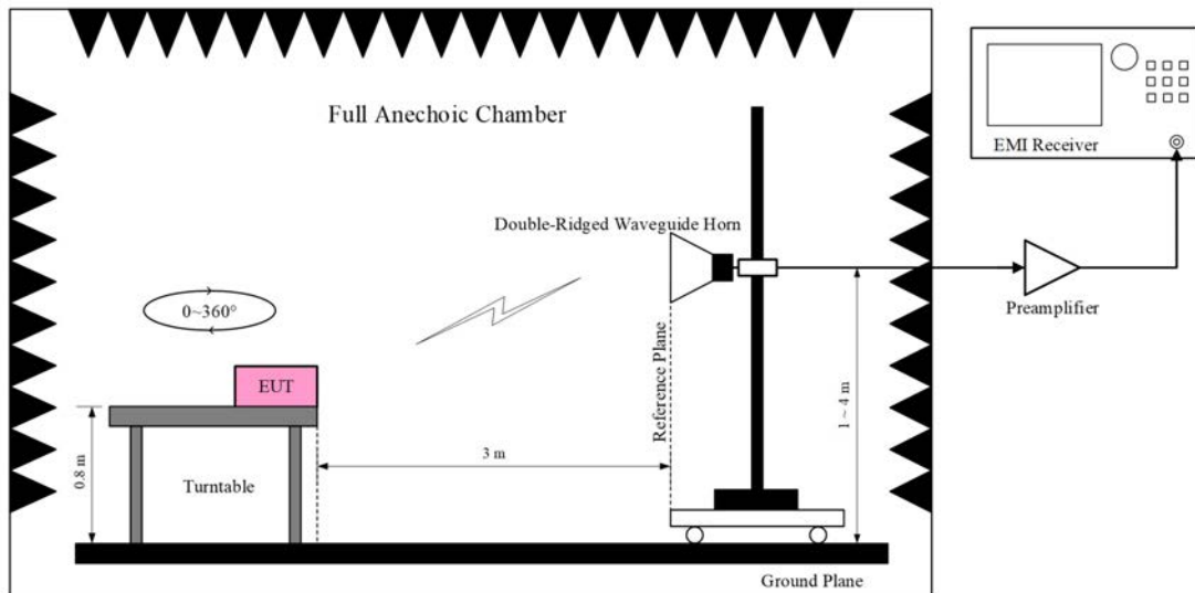
Figure 7-7: Test Configuration of Radiated Emissions Above 1 GHz
