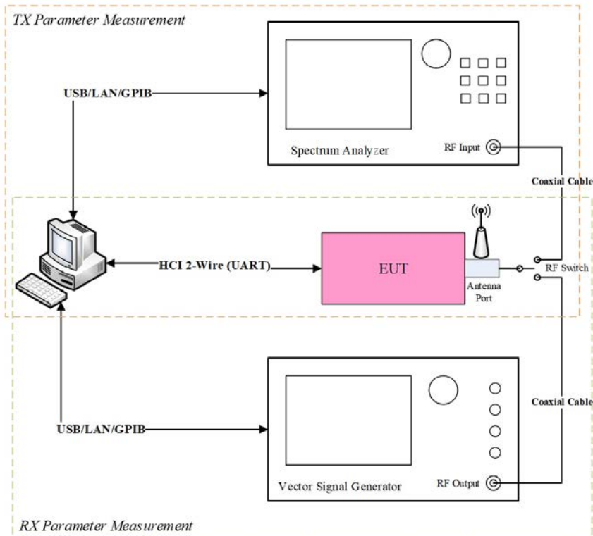
Figure 4-1: Brief Block Diagram of Conducted Test System
