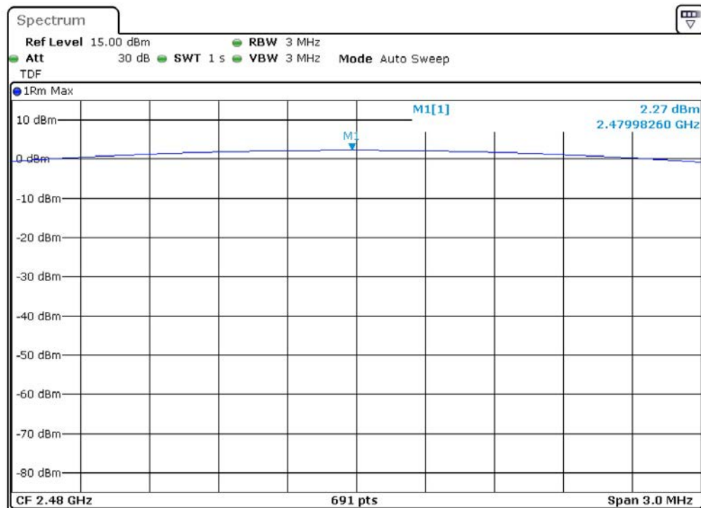
Figure 6-1: Example Test Plot of Peak Output Power Testing
