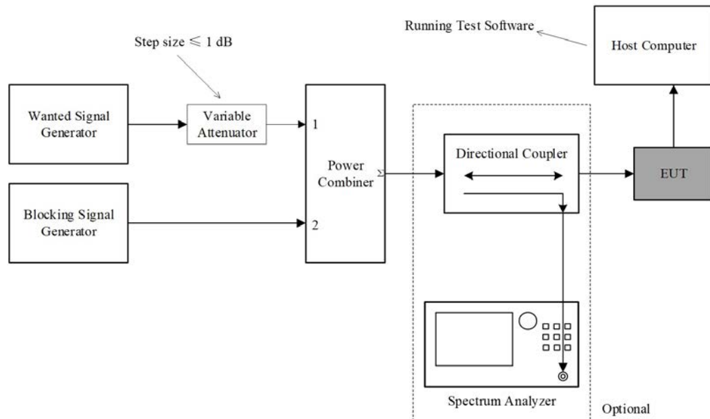
Figure 8-6: Test Setup for Receiver Blocking Measurements
