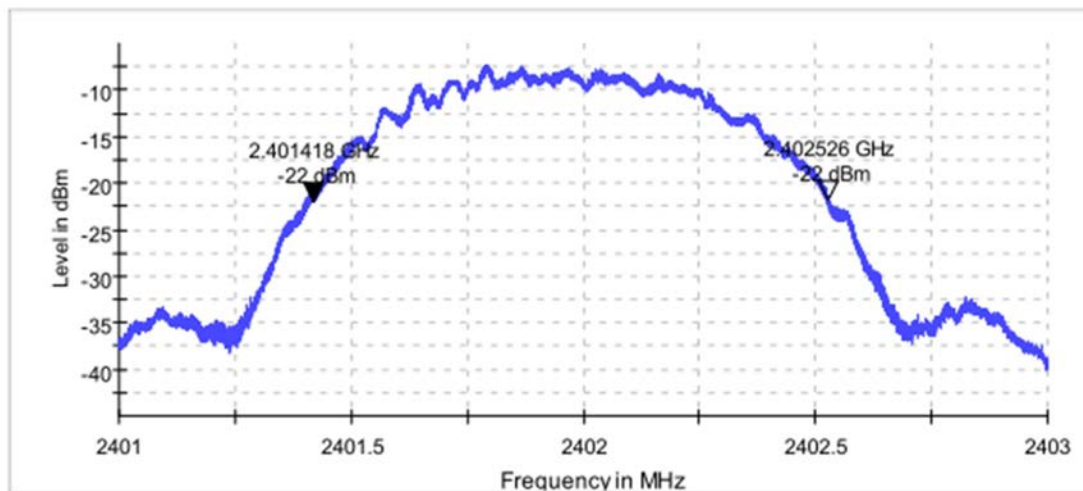
Figure 8-3: Example Test Plot of Occupied Channel Bandwidth of 2402 MHz
