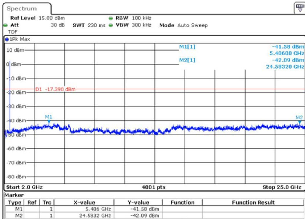
Figure 7-5: Example of Conducted Spurious Emission Test for 2 to 25 GHz
