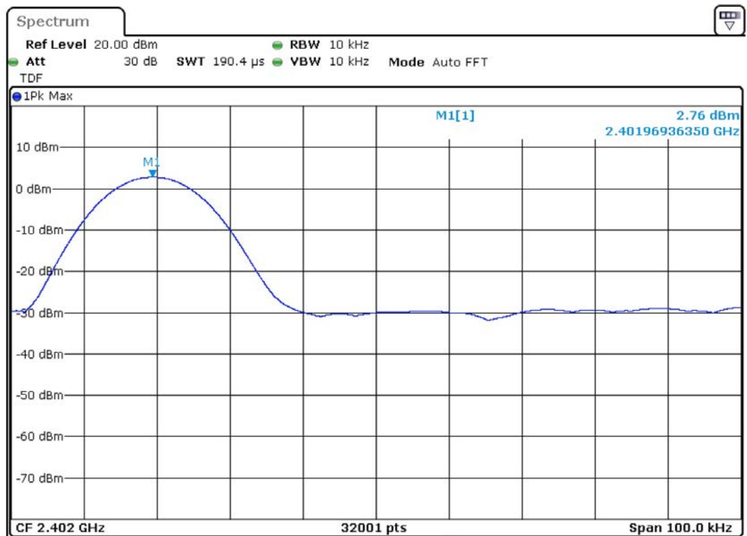
Figure 6-2: Example Test Plot of Frequency Tolerance Testing
