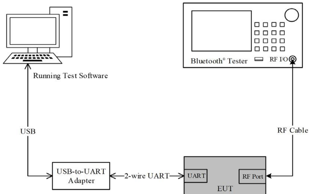
Figure 5-2: The Test Setup for Bluetooth Low Energy Non-Signaling Test Method
