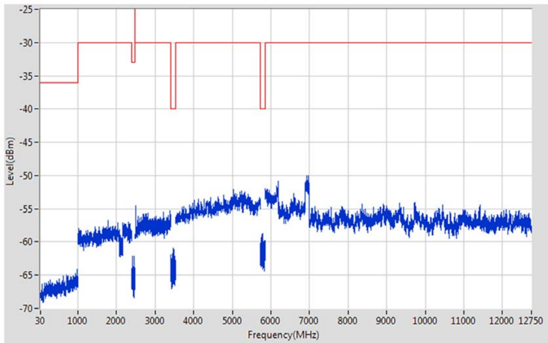
Figure 6-5: Example Test Plot of Collateral Emissions of Receiver
