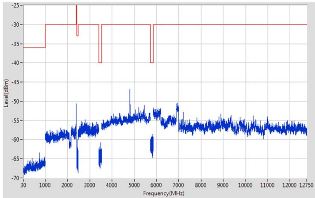
Figure 6-4: Example Test Plot of Collateral Emissions of Transmitter
