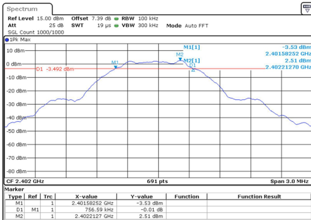
Figure 7-2: Example Test Plot of Occupied Bandwidth in Low Channel
