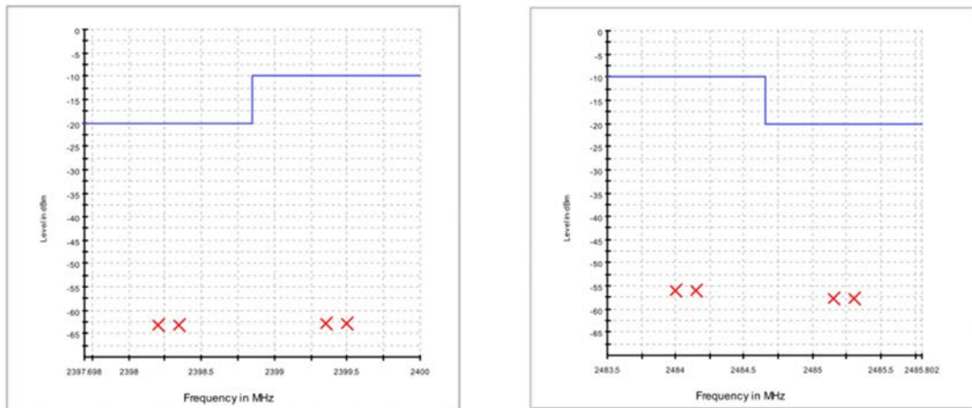
Figure 8-5: Example Test Plot of OOB Emissions While Operating at Highest Frequency
