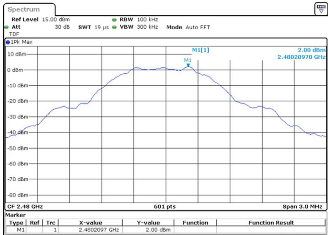
Figure 7-3: Example Test Plot of Fundamental Emission in High Channel
