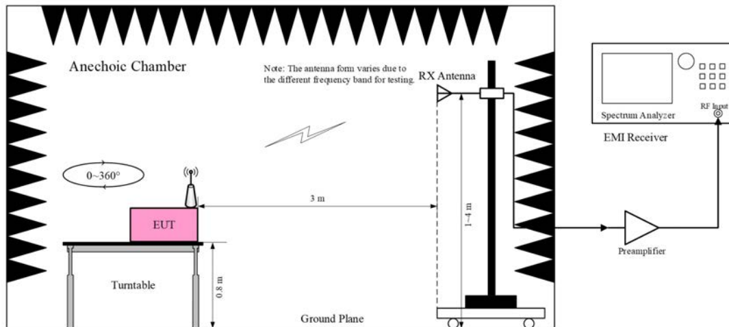
Figure 4-2: Brief Block Diagram of Typical Radiated Test System
