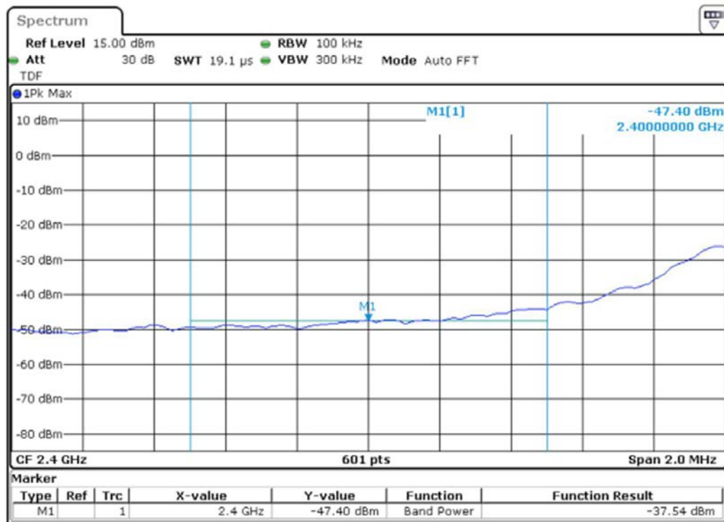
Figure 7-11: Band Power Integral Over 1 MHz Relative to Emission Frequency
