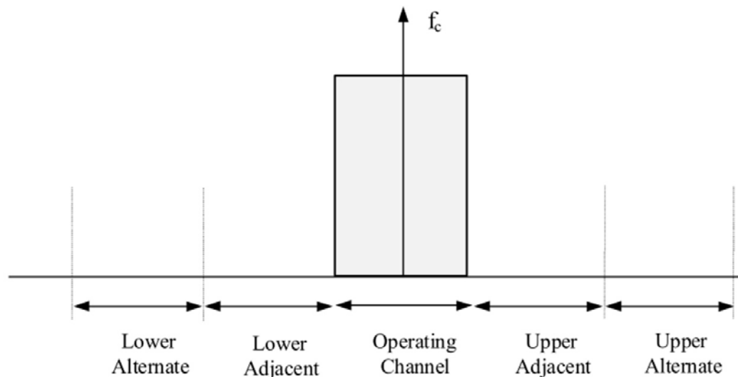
Figure 3-1: Adjacent and Alternate Channel Definitions
