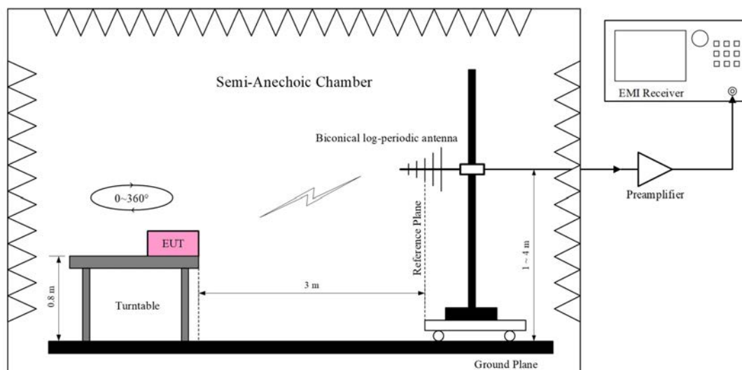
Figure 7-6: Test Configuration of Radiated Emission Below 1 GHz
