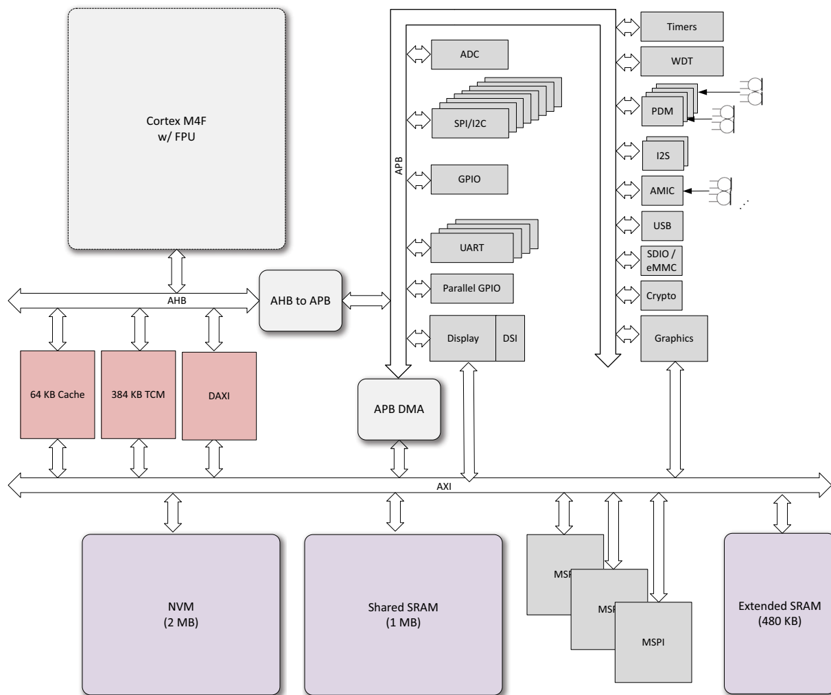
Figure 4. Apollo4 Blue SoC Peripherals, Memory and Buses
