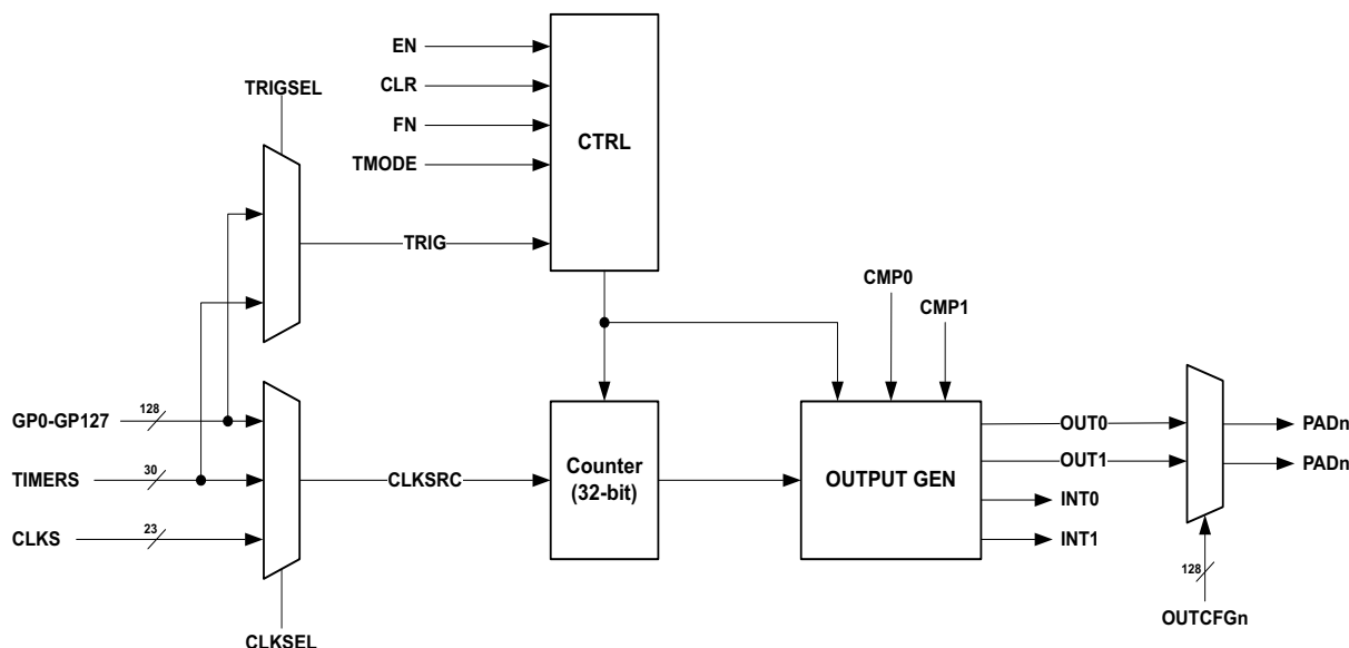
Figure 19. Block Diagram for One Counter/Timer
