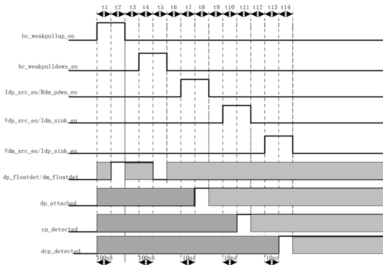
Figure 41. Battery Charging Sequence
