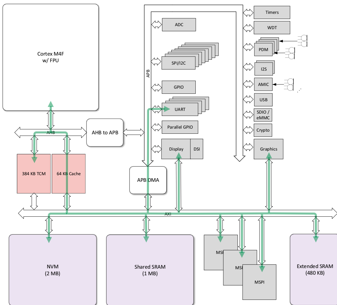
Figure 8. Apollo4 Blue SoC System Diagram
