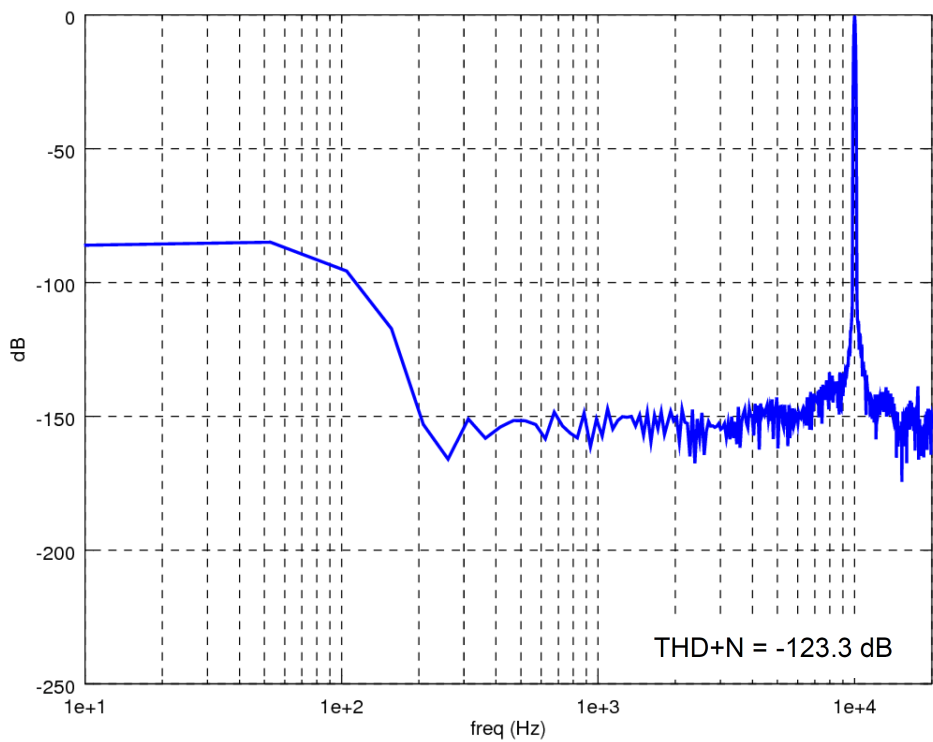
Figure 69. ASRC Performance Analysis - Test Case 4
