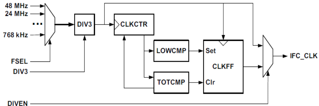
Figure 28. IO_CLK Generation
