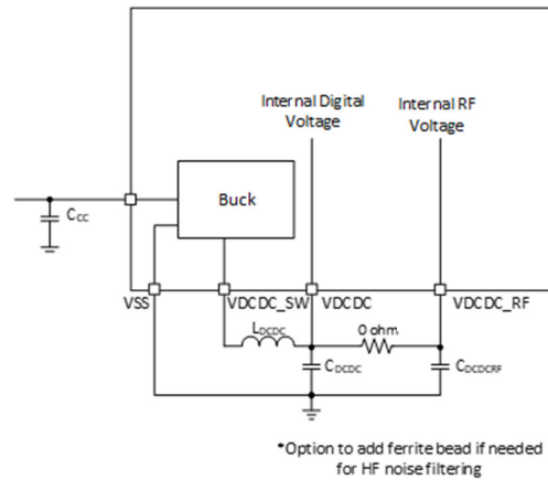
Figure 17. Integration Diagram for Buck Enabled Configuration
