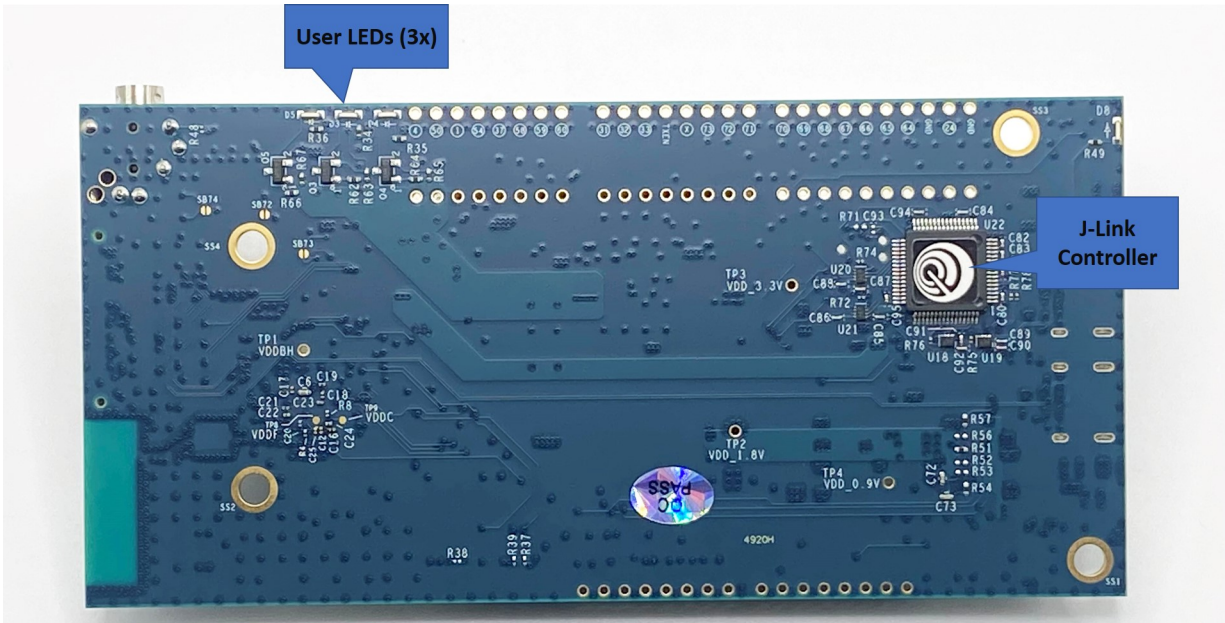
Figure 3. Apollo4 Blue Plus (KBR) Plus EVB - Major Bottom Side Components
