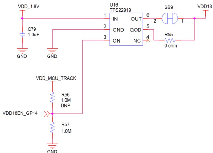
Figure 10. Apollo4 Blue Plus (KBR) EVB VDD18 Load Switch Circuit
