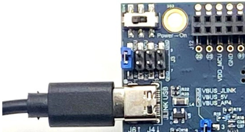
Figure 6. Apollo4 Blue Plus (KXR) EVB Using On-board J-Link Debugger
