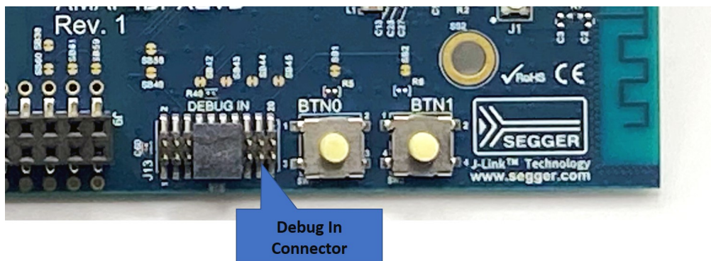
Figure 7. Apollo4 Blue Plus (KXR) EVB's DEBUG IN Header (J13)
