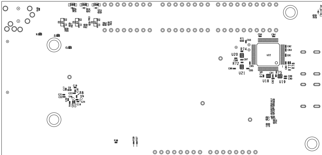
Figure 5. Apollo4 Blue Plus (KXR) Plus EVB - Bottom Side Parts Location
