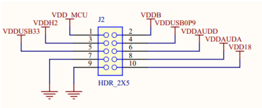
Figure 11. Apollo4 Blue Plus (KXR) EVB Voltage Test Points on Header J2
