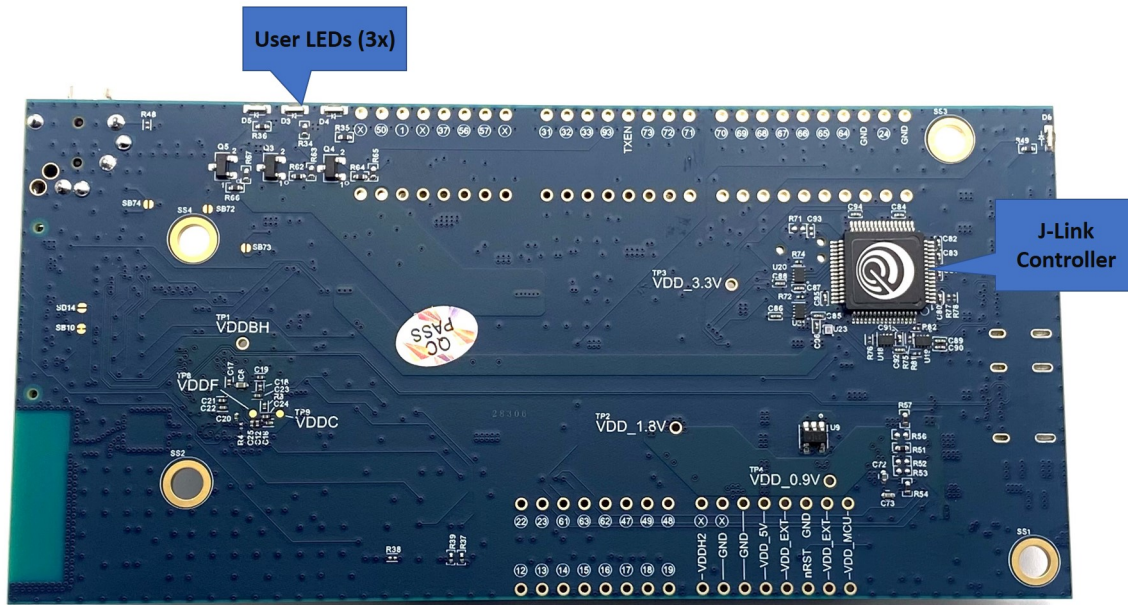
Figure 3. Apollo4 Blue Plus (KXR) Plus EVB - Major Bottom Side Components
