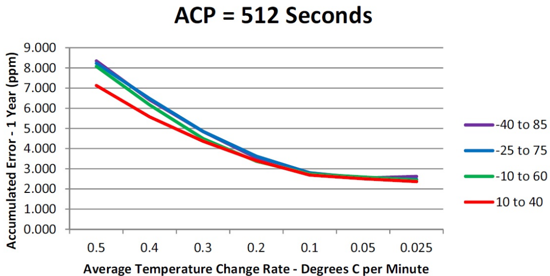
Figure 3-2: Autocalibration Error, ACP = 512 Seconds
