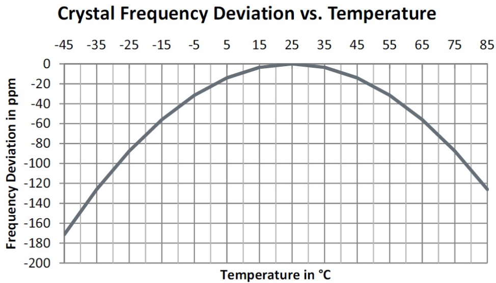
Figure 3-4: Typical Tuning Fork Crystal Frequency Deviation
