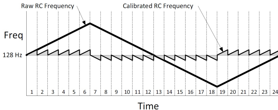
Figure 3-1: Autocalibration Error Cancellation
