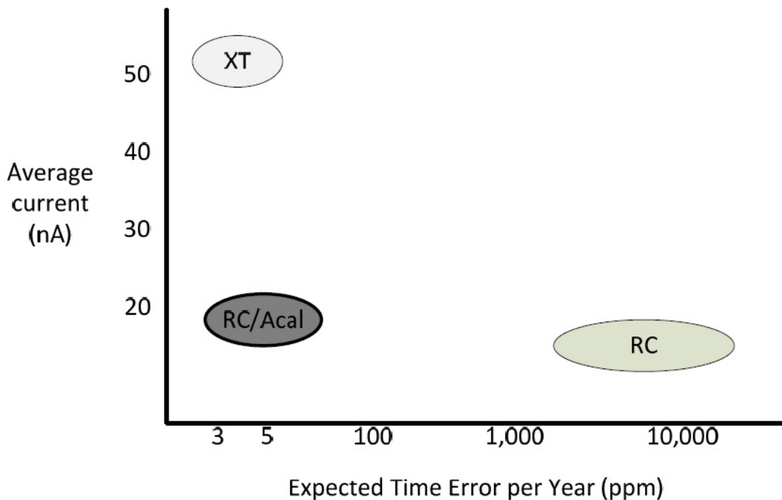
Figure 1-1: Base Mode Comparison
