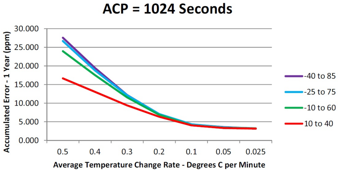
Figure 3-3: Autocalibration Error, ACP = 1024 Seconds
