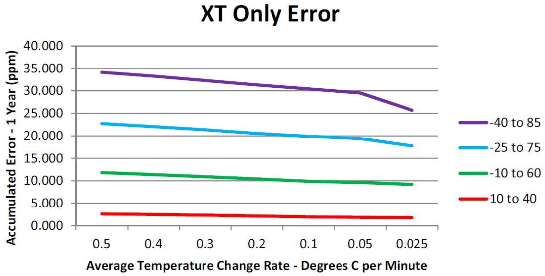
Figure 3-5: Raw Error, XT Oscillator
