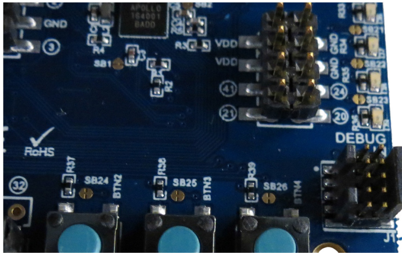
Figure 3-2: Apollo2 EVB's Cortex DEBUG IN Header (J1)
