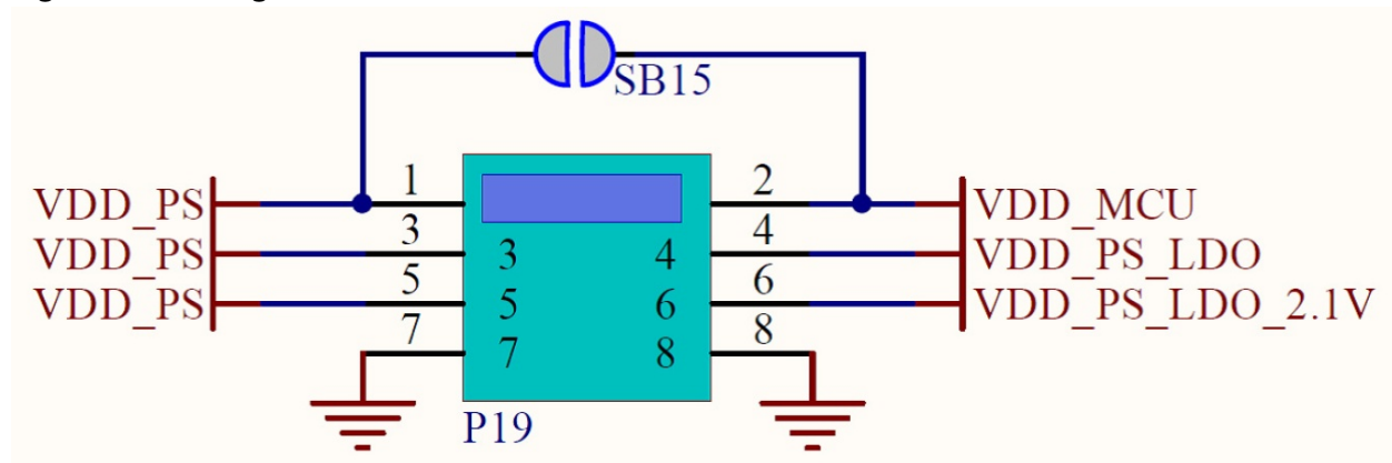
Figure 5-1: Voltage Selection on Header P19
