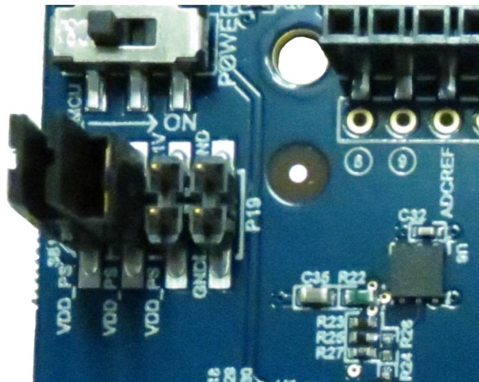
Figure 5-2: Header P19 Configured for 3.3V Operation - No Current Measurement
