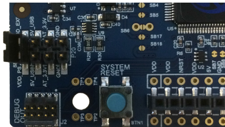
Figure 3-3: Apollo2 EVB's DEBUG OUT Header (J2)
