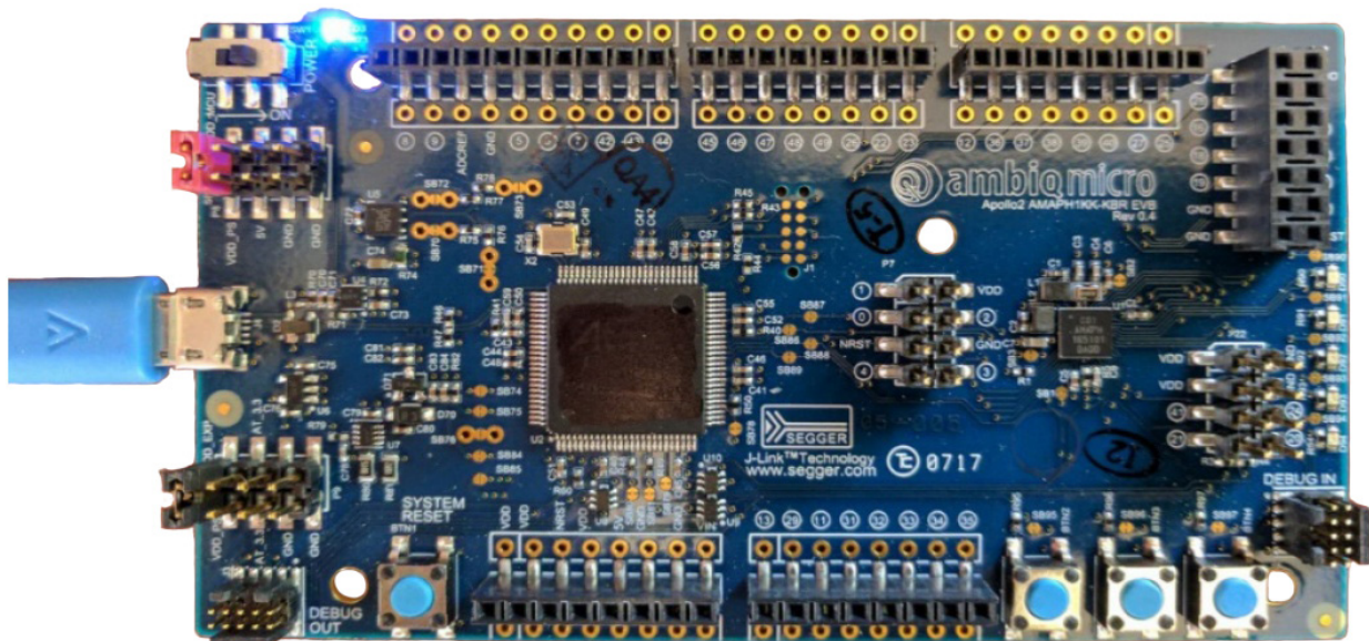
Figure 3-1: Apollo2 EVB Using On-board J-Link Debugger
