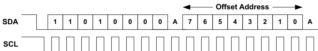
Figure 28. I²C Offset Address Transmission
