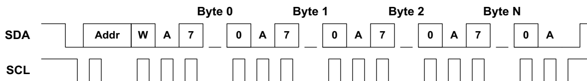
Figure 31. I²C Write Operation with No Address Offset
