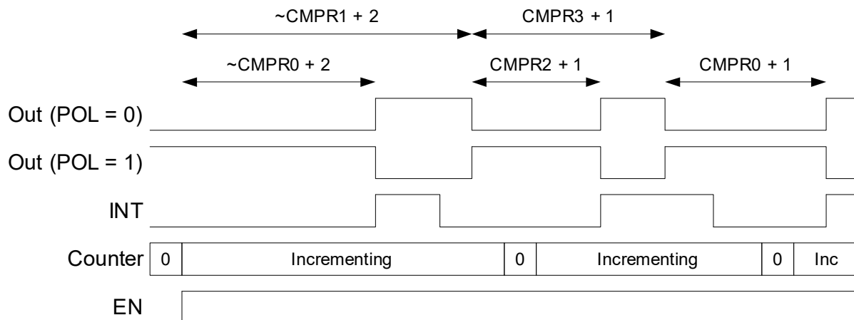
Figure 73. Counter/Timer Operation, FN = 7
