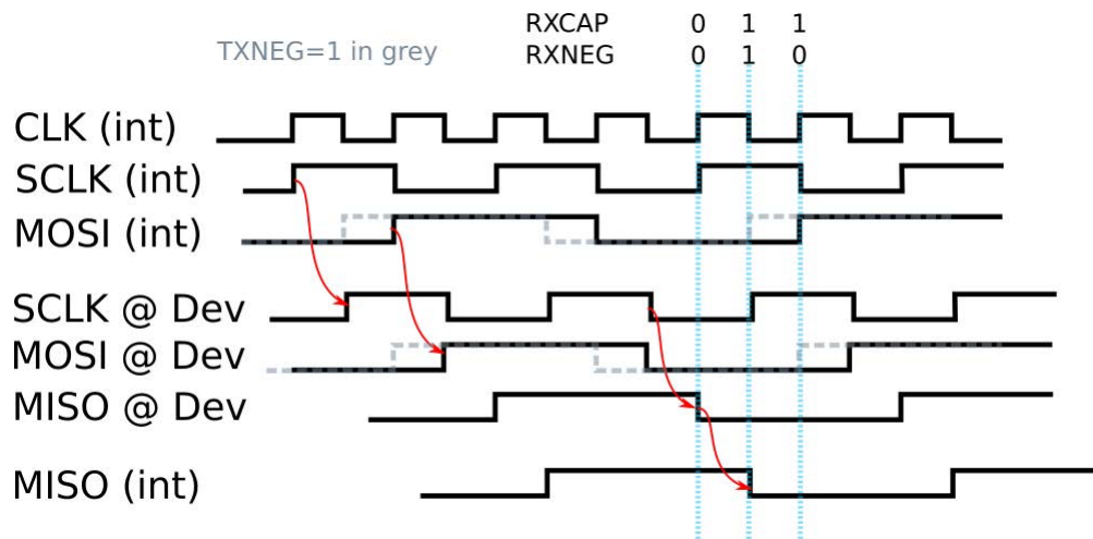
Figure 14. MSPI Interface Diagram
