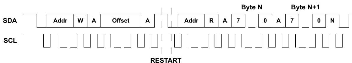
Figure 30. I²C Read Operation with Address Offset
