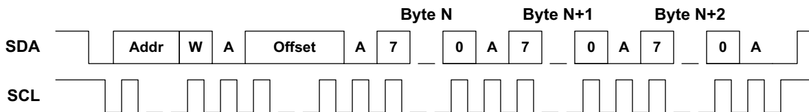
Figure 51. I²C Write Operation
