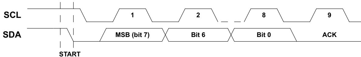
Figure 25. I 2 C Acknowledge
