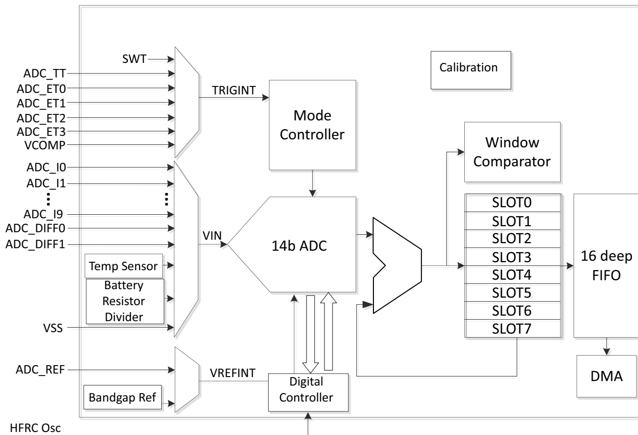
Figure 92. Block Diagram for ADC and Temperature Sensor
