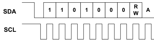
Figure 26. I²C 7-bit Address Operation
