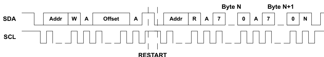
Figure 52. I²C Read Operation
