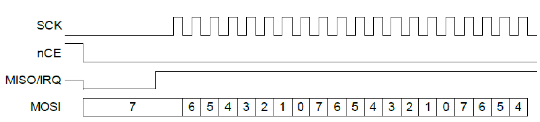
Figure 39. Flow Control at Beginning of a Write Transfer
