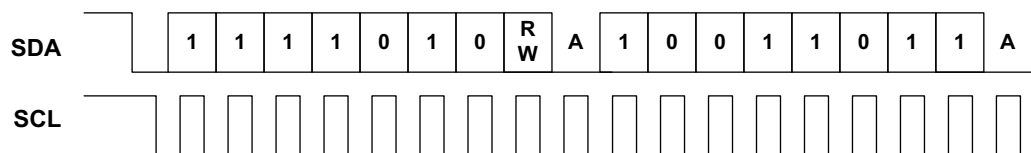
Figure 49. I 2 C 10-bit Address Operation
