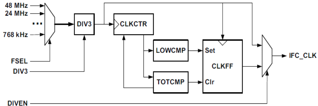
Figure 17. IO_CLK Generation
