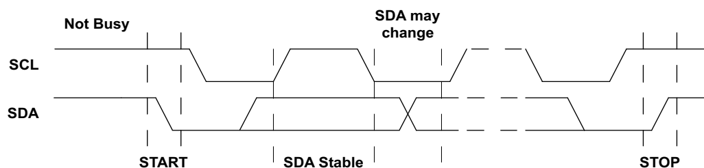
Figure 24. Basic I 2 C Conditions
