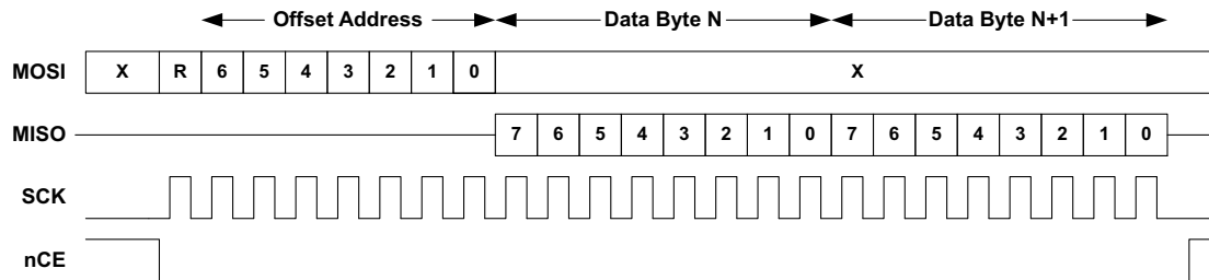
Figure 34. SPI Normal Read Operation
