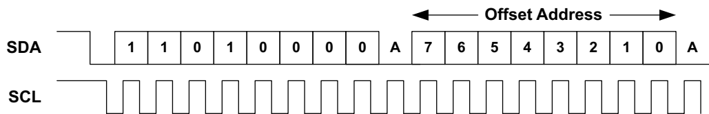
Figure 50. I²C Offset Address Transmission
