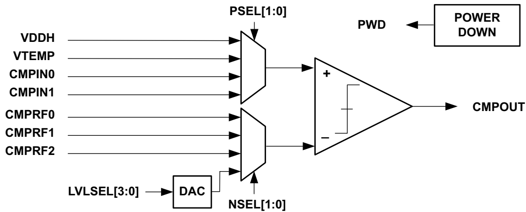
Figure 95. Block diagram for the Voltage Comparator Module
