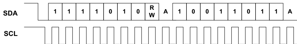
Figure 27. I²C 10-bit Address Operation
