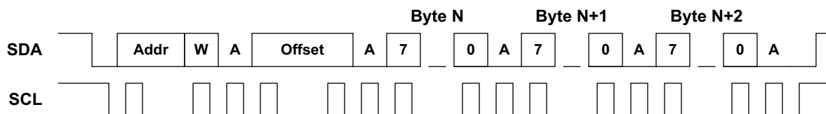
Figure 29. I²C Write Operation with Address Offset
