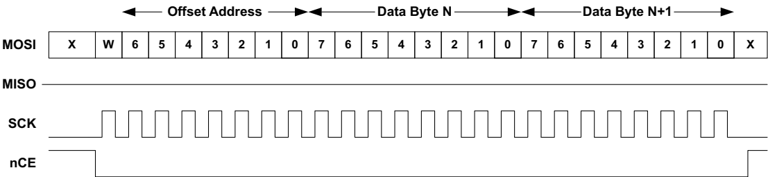
Figure 33. SPI Normal Write Operation (Single-byte Offset Address)
