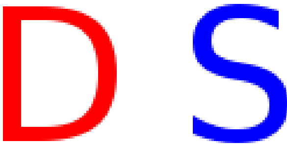
Figure 10: Scene Textures
