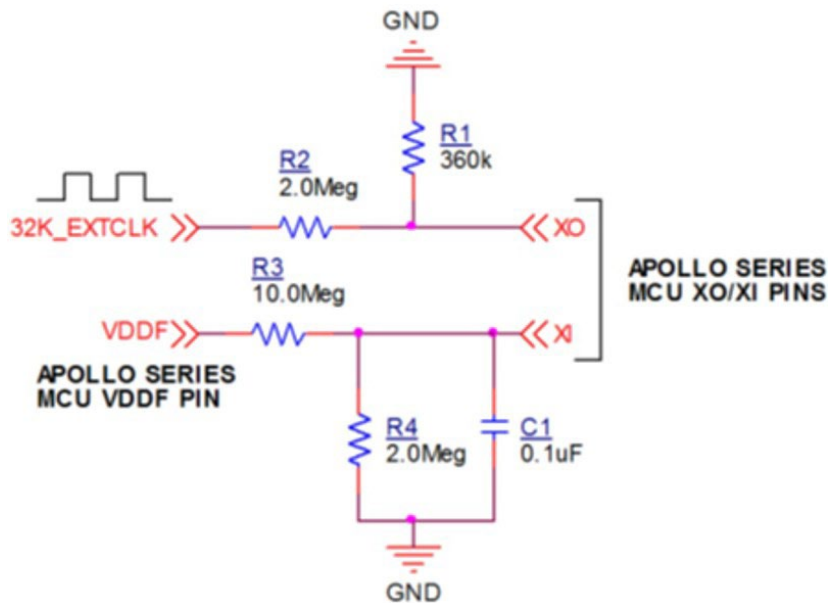
Figure 8-1: 32.768 kHz Crystal Clock Circuit Diagram
