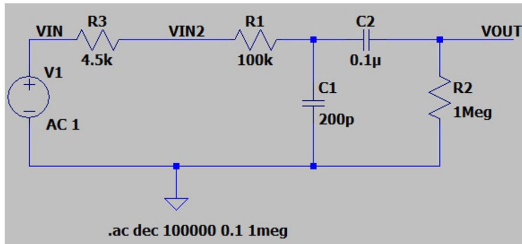
Figure 12-4: Simulated Circuit
